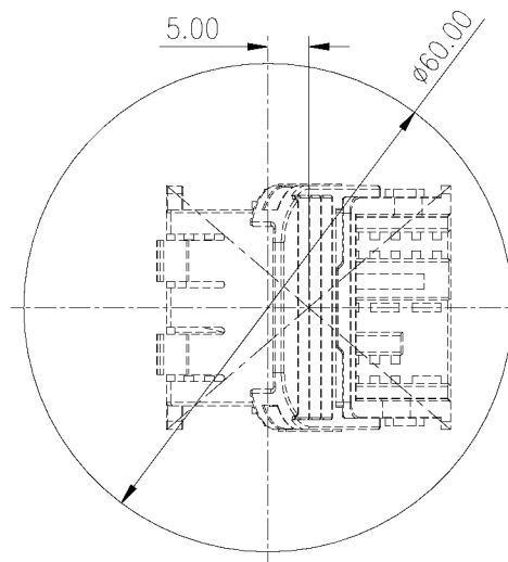
Recommended cut-out diameter dimension
