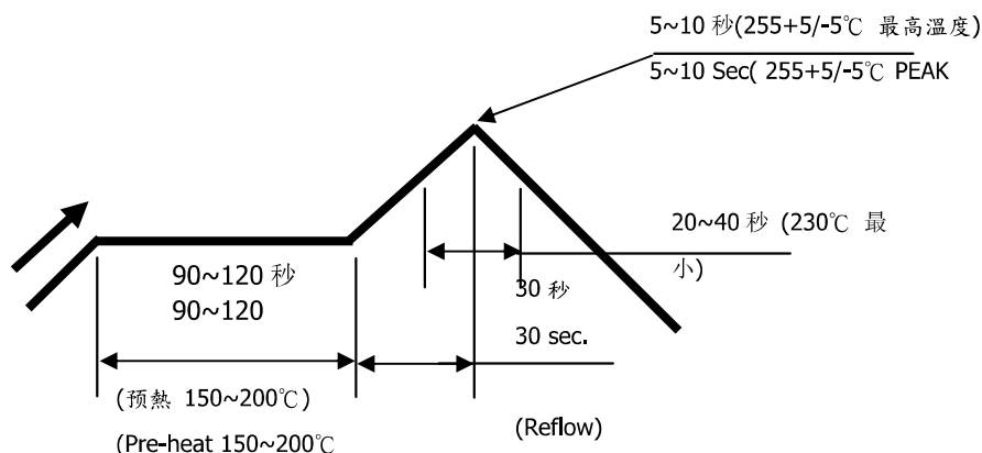
温度条件曲线图/ 基板上温度 TEMPERATURE CONDITION GRAPH/ (TEMPERATURE ON BOARD PATTERN SIDE)
